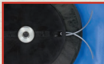
FLEXIBLADE CUTTING SYSTEM Cutting line with solid core and serrated edges
